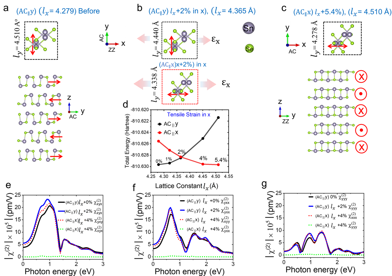
Figure 4. Theoretical characterization of five-layer SnSe with AB stacking. (a) Top and side views of the strain-free structure for the state (AC_{||}y) . (b) Top views of the structures for the states (AC_{||}y) and (AC_{||}x) , respectively under the strain condition with a fixed lattice constant along x with l_x = 4.365 Å. (c) Top and side views of the strain-free structure for the state (AC_{||}x) . (d) Total energy of the structures of (AC_{||}y) and (AC_{||}x) as a function of l_x . The absolute values of SHG susceptibility spectra of (e) \chi_{xyx}^{(2)}(\chi_{xyx}^{(2)}) , (f) \chi_{yxx}^{(2)}(\chi_{xyy}^{(2)}) , (g) \chi_{yyy}^{(2)}(\chi_{xxx}^{(2)}) under different strain conditions.
