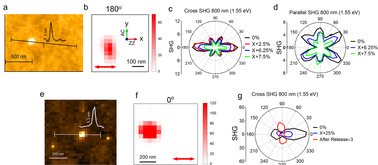
Figure 2. Experimental characterization of few-layer SnSe flakes. (a) AFM image of a SnSe flake on a PDMS substrate. (b) SHG image of the same SnSe flake in (a), recorded at a sample rotational angle of 180^\circ . The red arrow indicates the polarization direction of the incident laser. (c) Cross-polarized and (d) parallel-polarized SHG intensity of the flake in (b) as a function of rotational angle. The different colors correspond to SHG polar patterns under various tensile strains applied along the x -axis of the SnSe. (e) AFM image of another SnSe flake on a PDMS substrate. (f) SHG image of the SnSe flake in (e), acquired at a sample rotational angle of 0^\circ . (g) Cross-polarized SHG intensity of the flake in (f) as a function of rotational angle. The red line indicates the SHG intensity (scaled by a factor of 3) after the strain is released.
